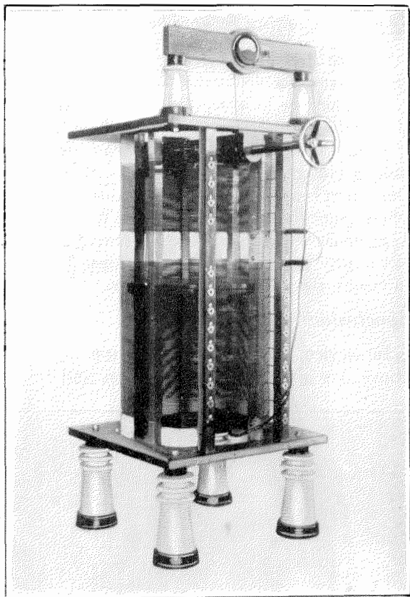
Figure 9—Antenna Tuning Coil.
