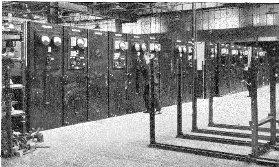
Figure 12—B. T. H. Truck Type Switchgear Units (Front View).
