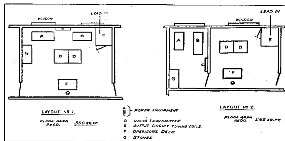
Figure 1—Typical Layouts.
