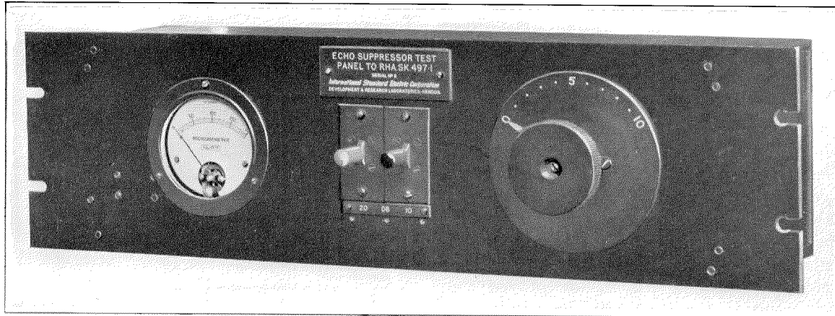
Figure 8—Testing Panel—Front View.
