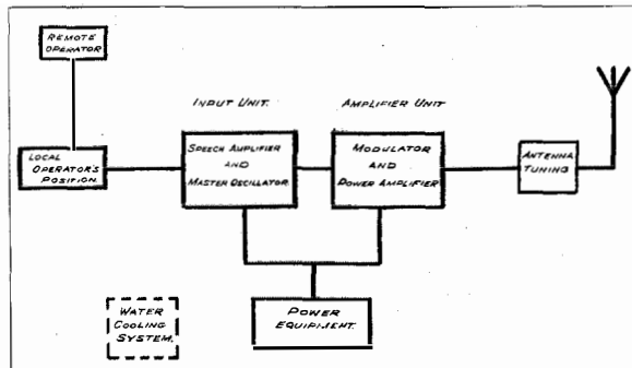
Figure 3—Block Schematic of Equipment.
