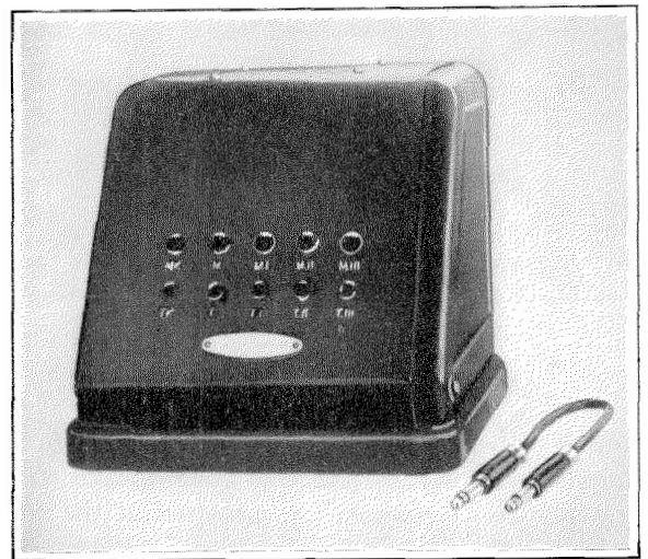
Figure 10—Switching Panel.
