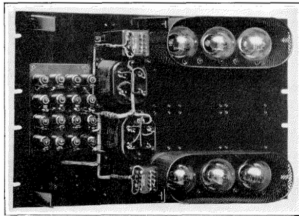
Figure 5—Front View of Echo Suppressor with Cover Removed.
