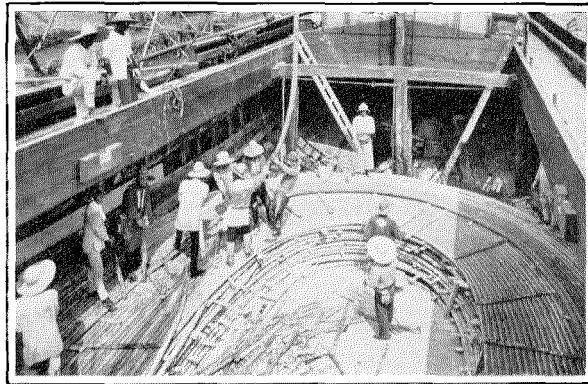
The Hold of the "TAISHO MARU" During the Loading Operations.
