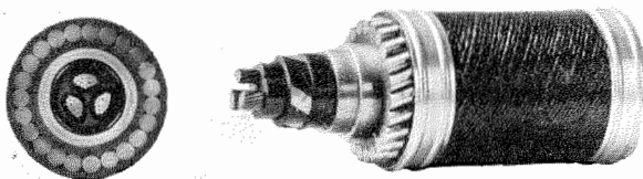
Shore End Cable—Telescoped End and Cross Section.
