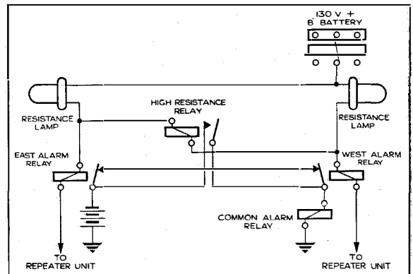
Figure 9—Modification of Repeater Alarm Circuit.
