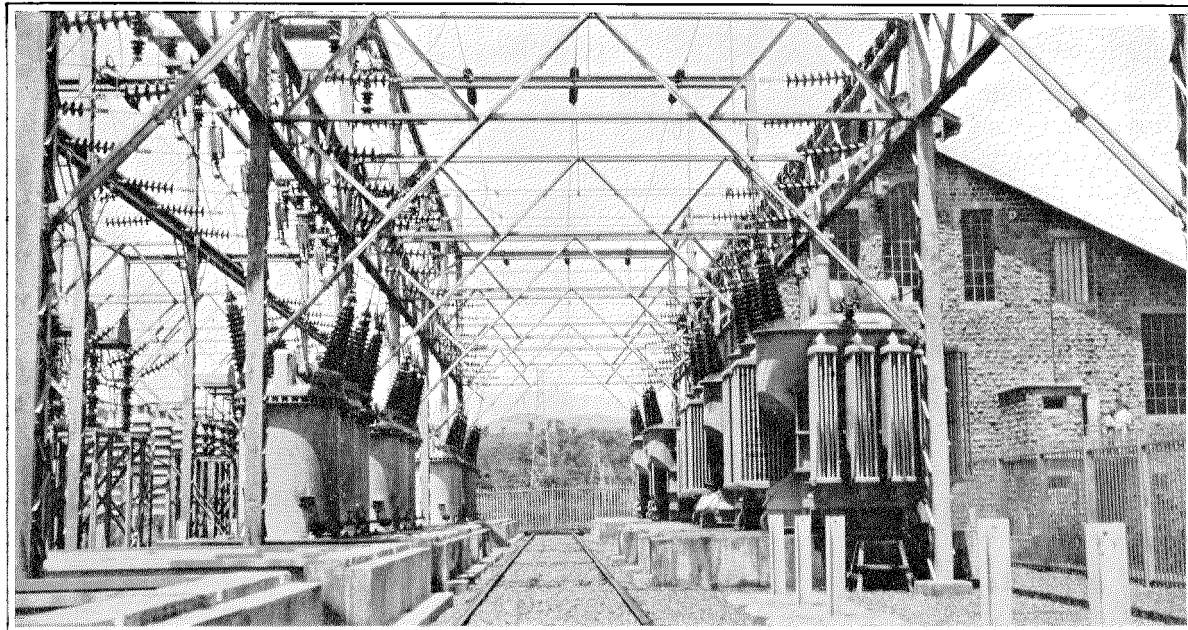
Figure 8—95 KV Outdoor Equipment at Karjat Substation.
