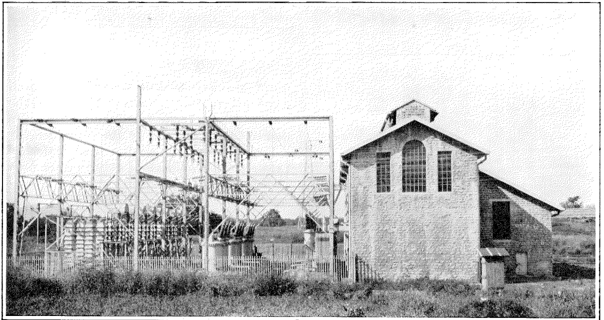
Figure 7—Vangani Substation.
