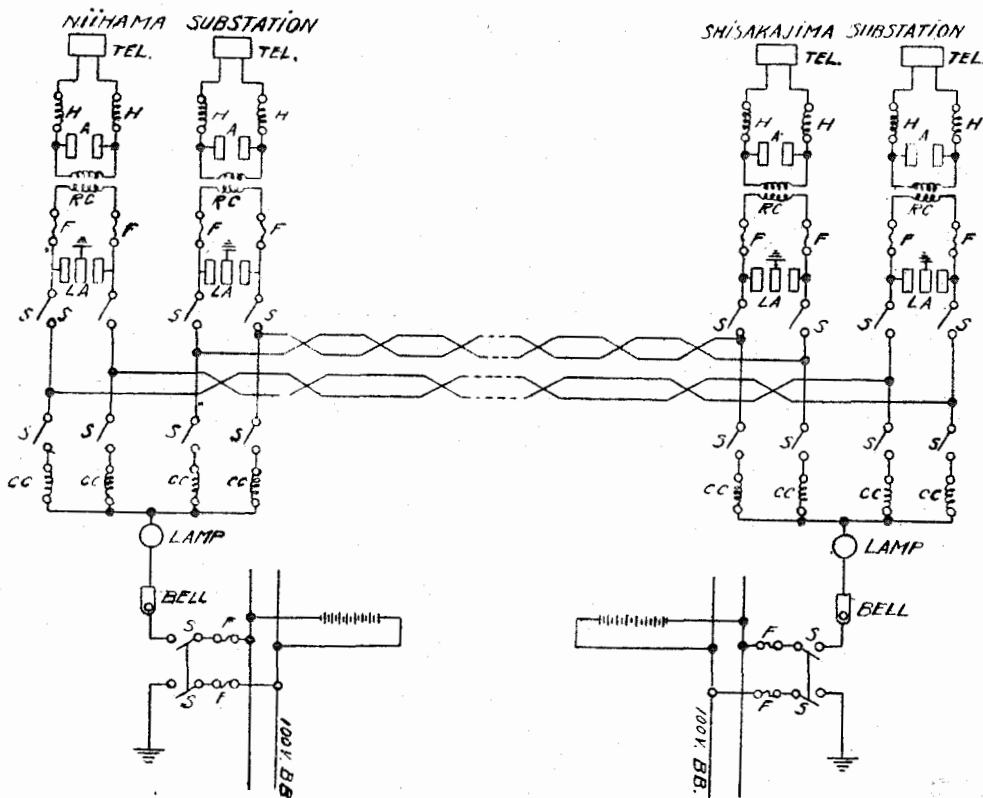
Schematic of Fault-Indicating and Telephone Circuits.
