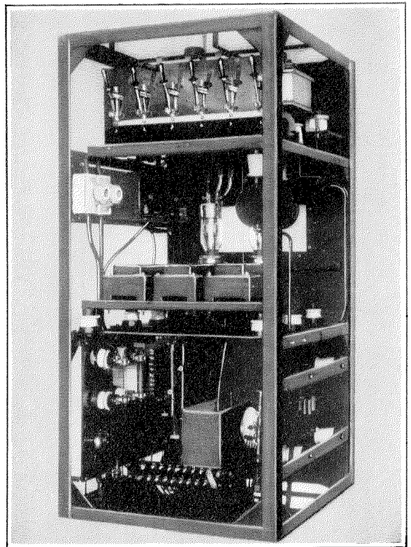
Figure 8—Rear View of Amplifier Unit 2/3.5 kw. Transmitter.
