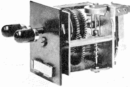
Figure 2—Selector Key.
